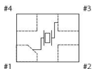
Land Pattern(REFERENCE)
