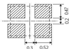
Land Pattern(REFERENCE)
